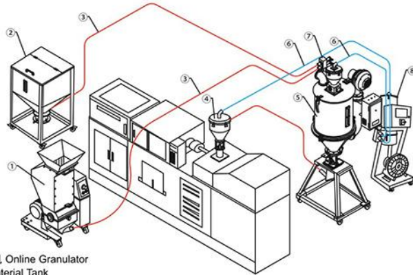
900G2吸料机应用（双段送料） 900G2 Application (Two-stage Conveying)
